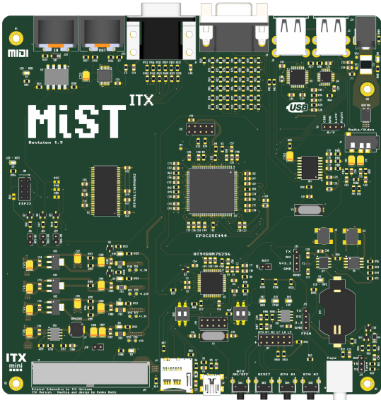
170.00 × 170.00 mm outline
