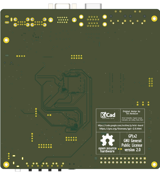
170.00 × 170.00 mm outline
